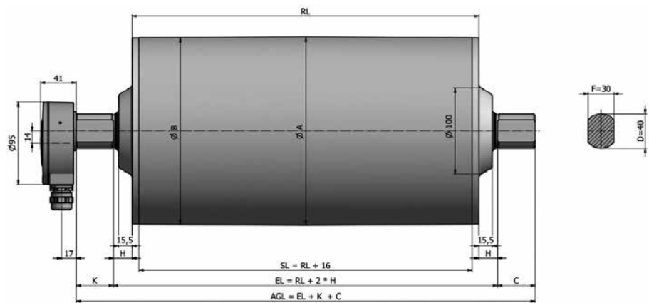
Drum motor standard version with terminal box in aluminium ≤ 4,0 kW
