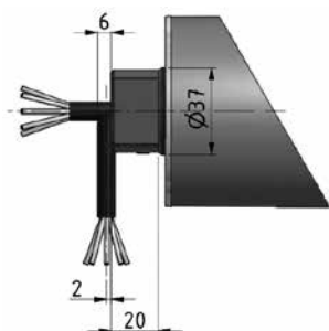
Shaft cap Uni in stainless steel
