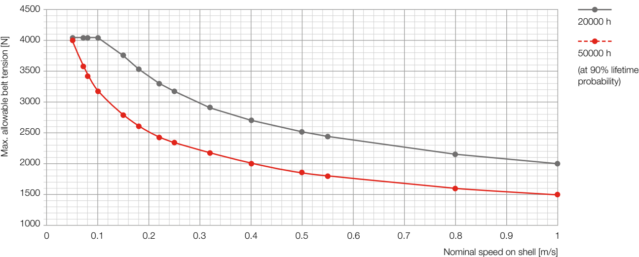
Belt tension diagram
