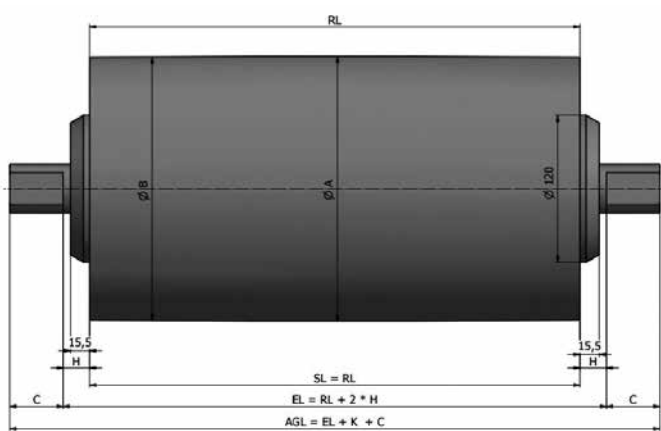
Idler Pulley in stainless steel (TS10N/TS12N)
