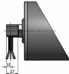
Cable slot 90° with threaded shaft
