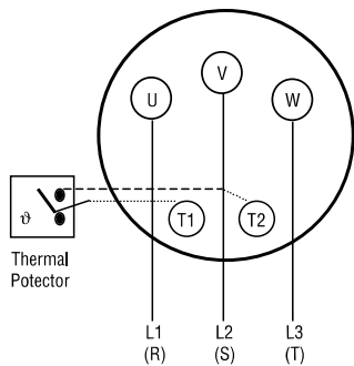
3-phase single voltage 5.5 kW
