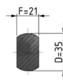
Shaft cap
