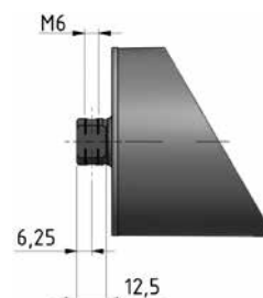
Cross-drilled and threaded shaft
