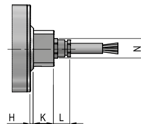
Straight connector
