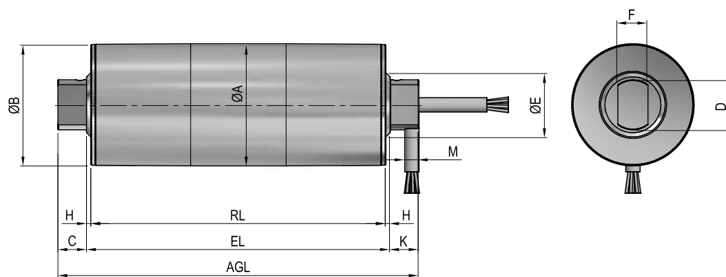
Drum motor Standard Version
