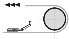
Plough cleaner type VLP
