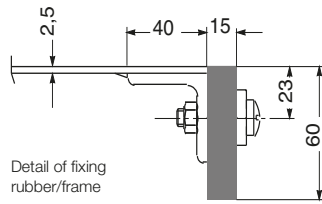
Plough cleaner type VLG
